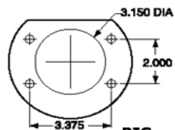
SMALL FORD BIG BEARING Axle housing (New)
